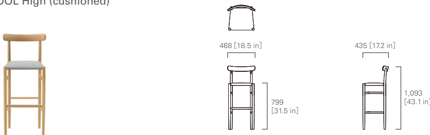
BAR STOOL High (cushioned)
