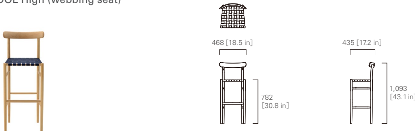
BAR STOOL High (webbing seat)
