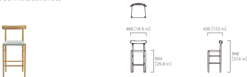
BAR STOOL Mid (cushioned)
