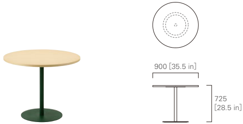
ROUND TABLE 90 (veneered top or solid wood top)
