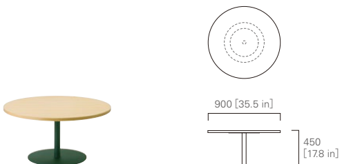
COFFEE TABLE 90 (veneered top or solid wood top)
