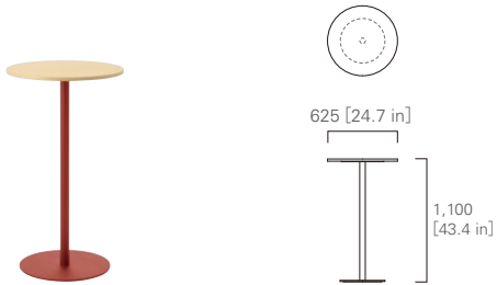
ROUND BAR TABLE 63 (veneered top)
