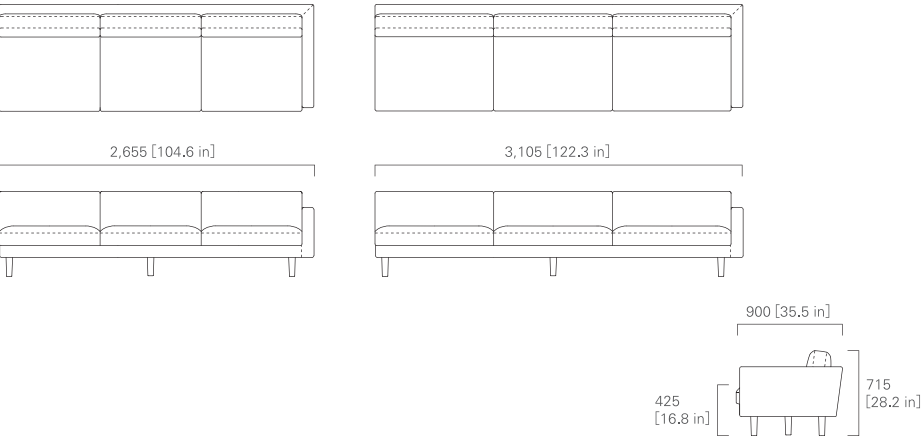
THREE SEATER SOFA Right
