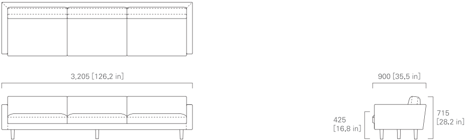
WIDE THREE SEATER SOFA
