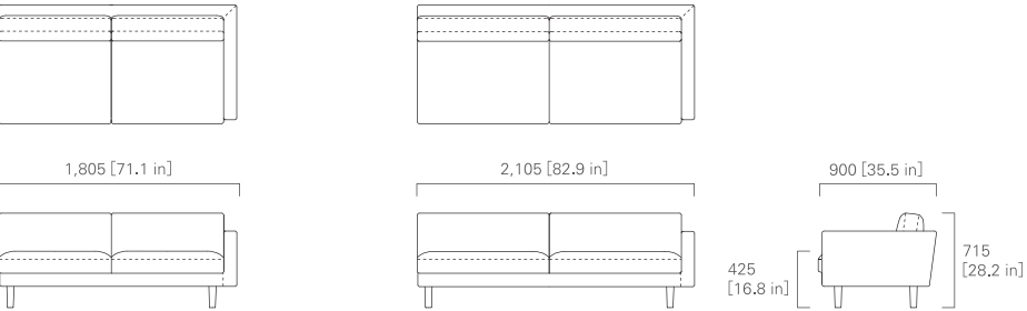
TWO SEATER SOFA Right
