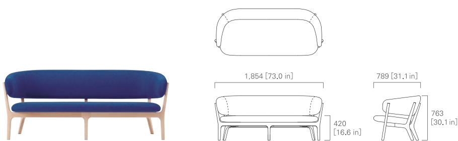
TWO SEATER SOFA
